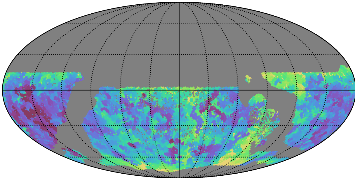
too_combined_s0.5_v3.4_10yrs WFD u band: Min seeingEff
