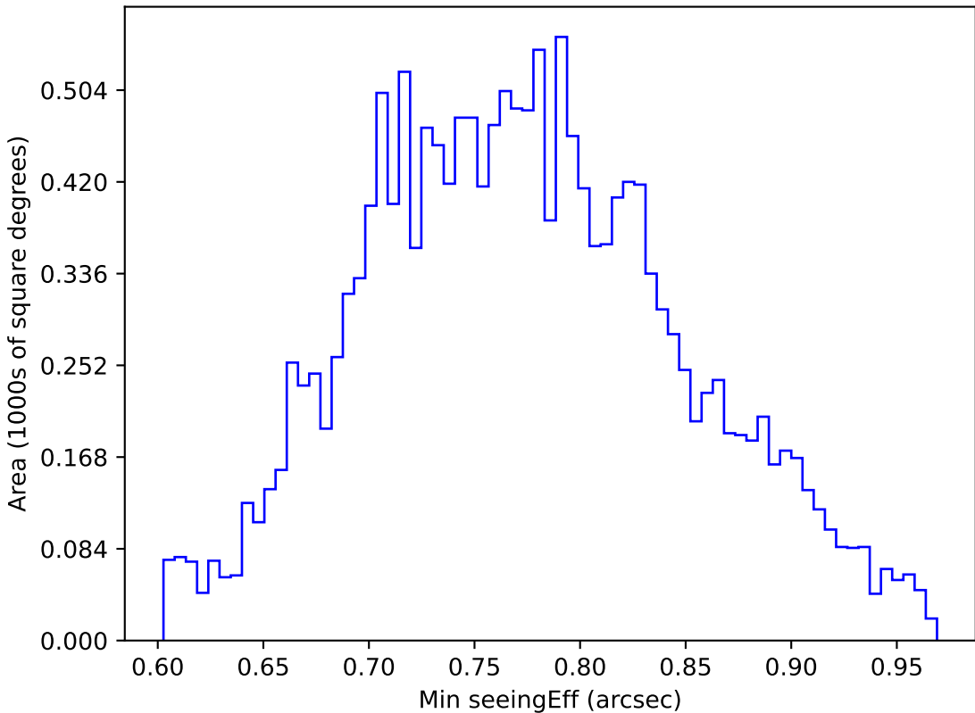
too_combined_s0.5_v3.4_10yrs WFD u band: Min seeingEff
