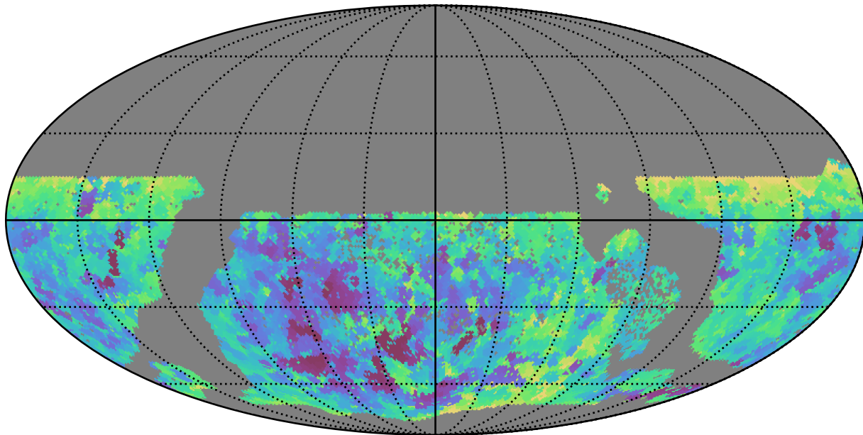
too_combined_s0.5_v3.4_10yrs WFD r band: Min seeingEff
