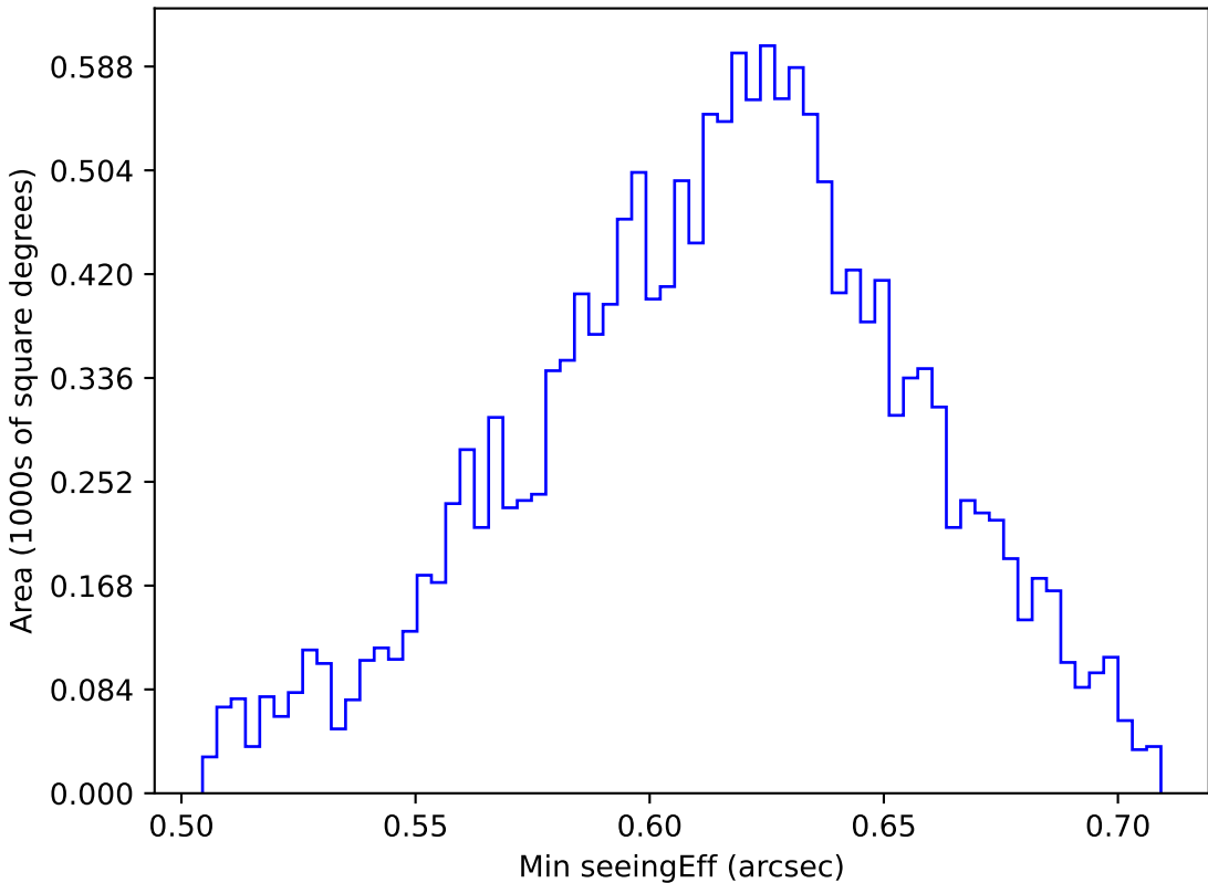
too_combined_s0.5_v3.4_10yrs WFD r band: Min seeingEff
