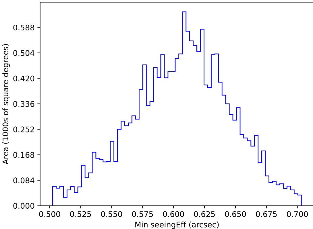
too_combined_s0.5_v3.4_10yrs WFD i band: Min seeingEff
