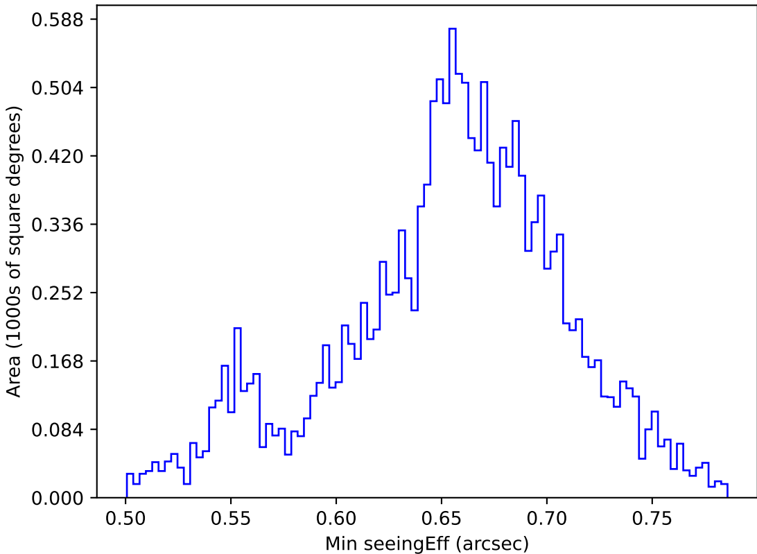
too_combined_s0.5_v3.4_10yrs WFD g band: Min seeingEff
