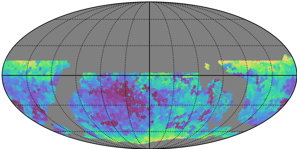
too_combined_s0.5_v3.4_10yrs WFD all bands: Min seeingEff
