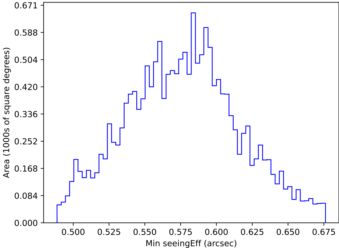
too_combined_s0.5_v3.4_10yrs WFD all bands: Min seeingEff
