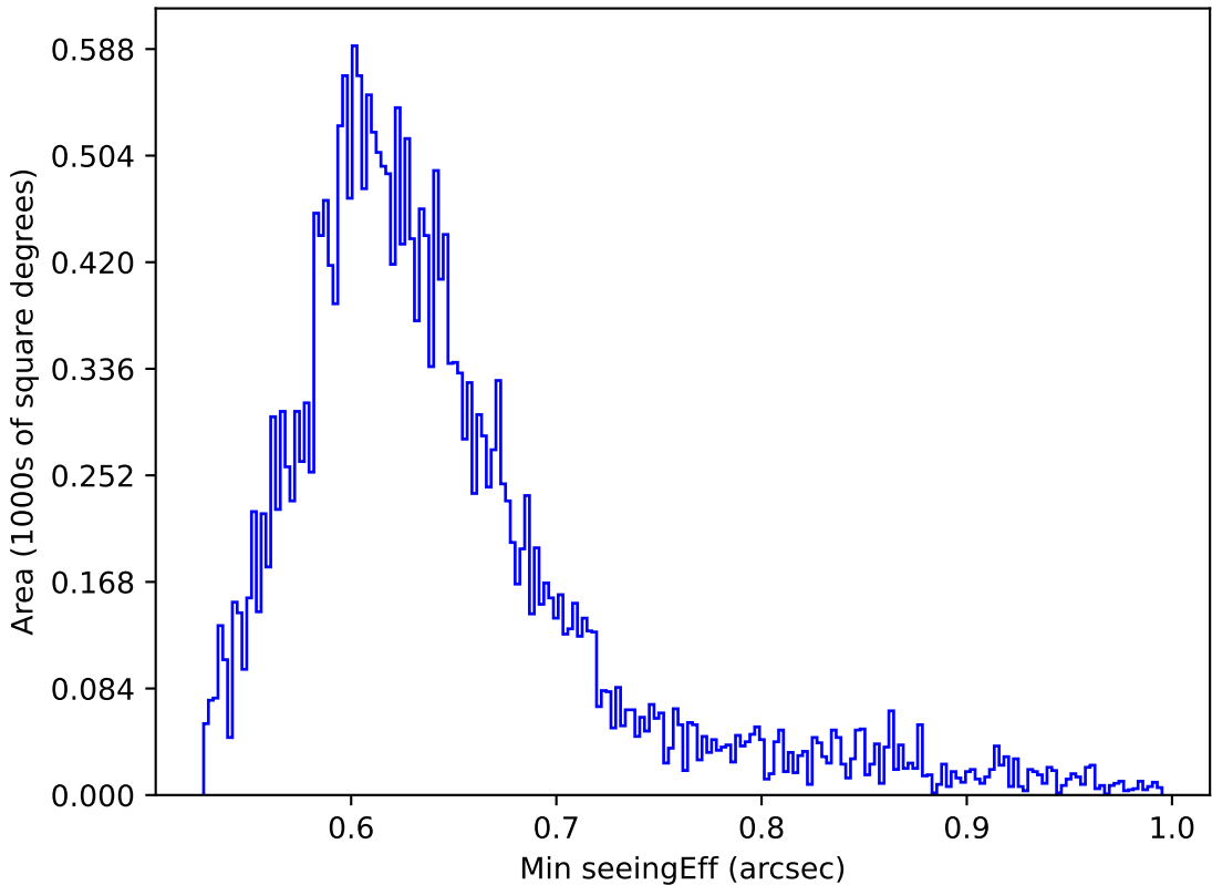
too_combined_s0.5_v3.4_10yrs All sky z band: Min seeingEff
