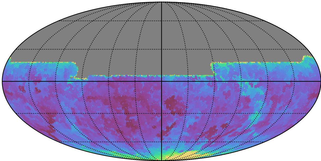
too_combined_s0.5_v3.4_10yrs All sky y band: Min seeingEff
