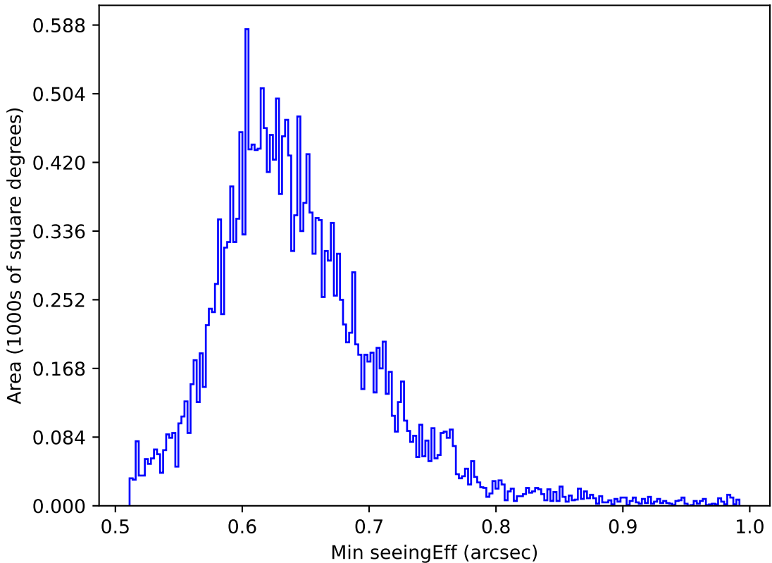
too_combined_s0.5_v3.4_10yrs All sky y band: Min seeingEff
