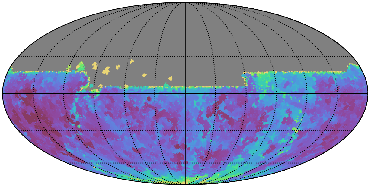
too_combined_s0.5_v3.4_10yrs All sky u band: Min seeingEff
