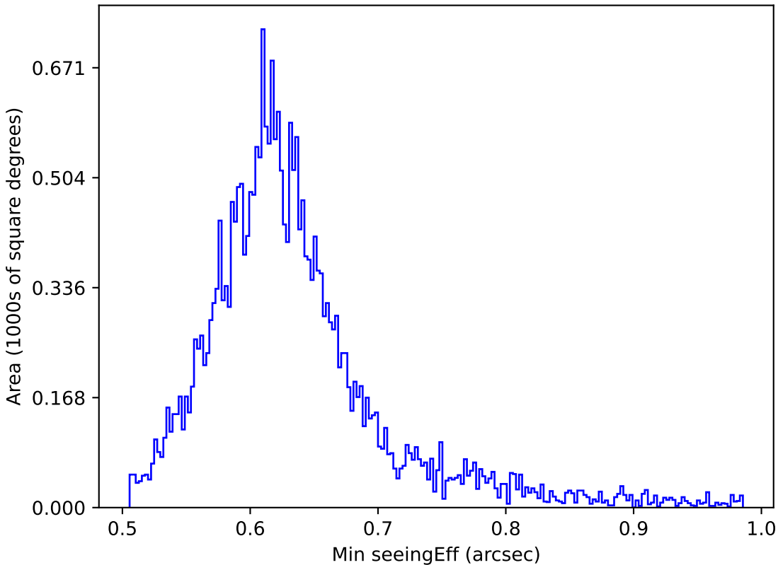
too_combined_s0.5_v3.4_10yrs All sky i band: Min seeingEff
