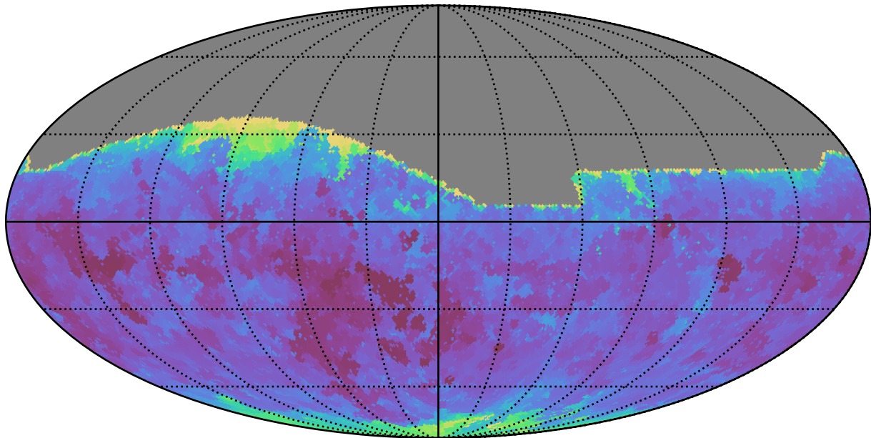
too_combined_s0.5_v3.4_10yrs All sky g band: Min seeingEff
