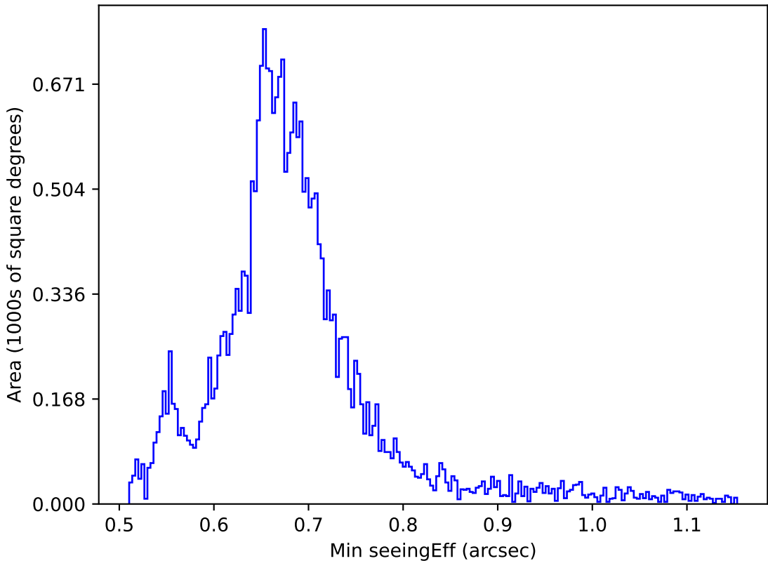
too_combined_s0.5_v3.4_10yrs All sky g band: Min seeingEff
