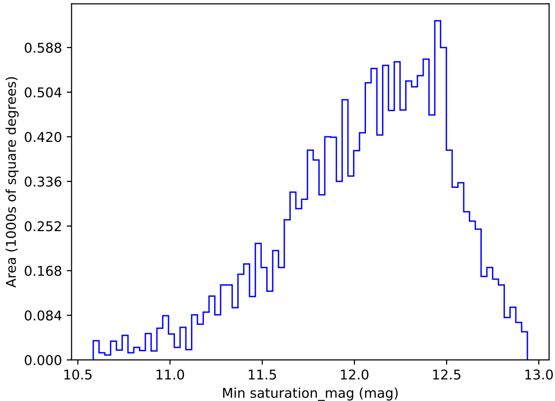
too_combined_s0.5_v3.4_10yrs WFD z band: Min saturation_mag
