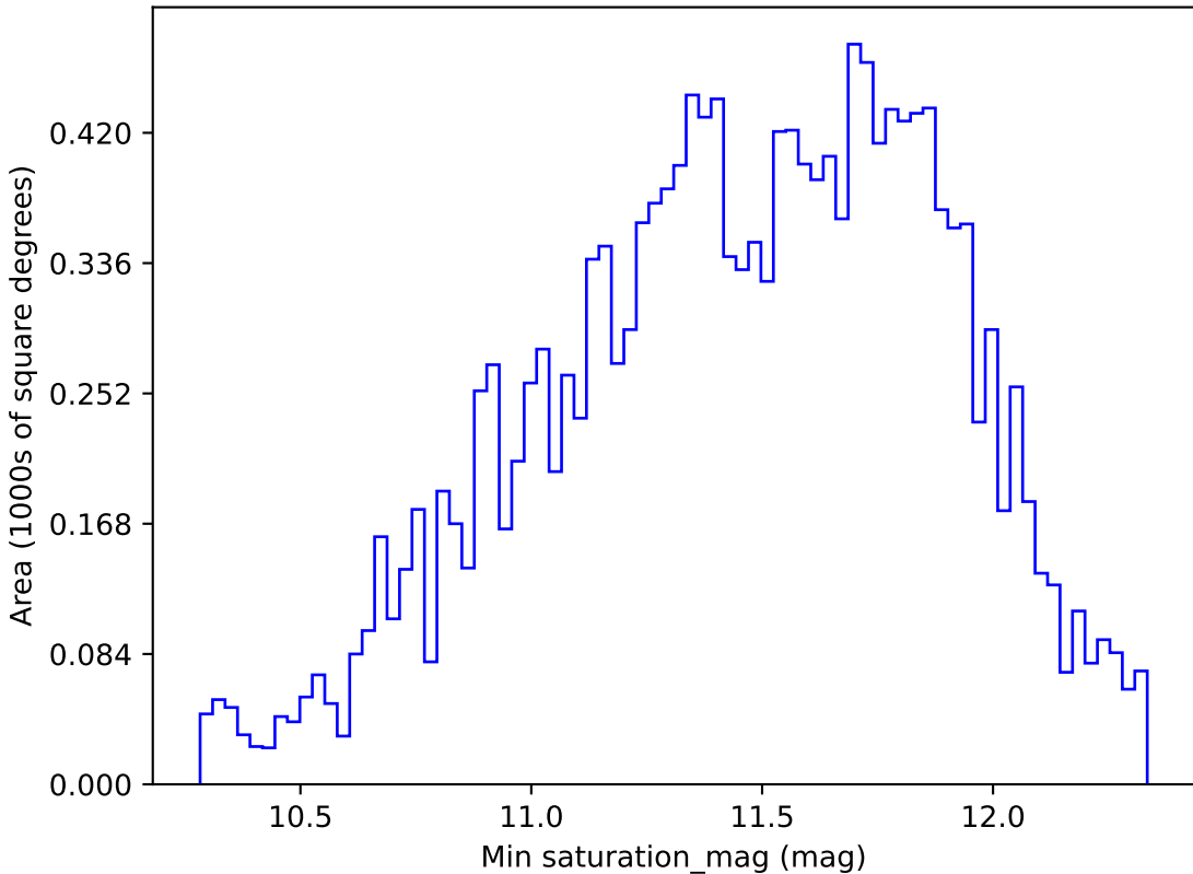
too_combined_s0.5_v3.4_10yrs WFD u band: Min saturation_mag
