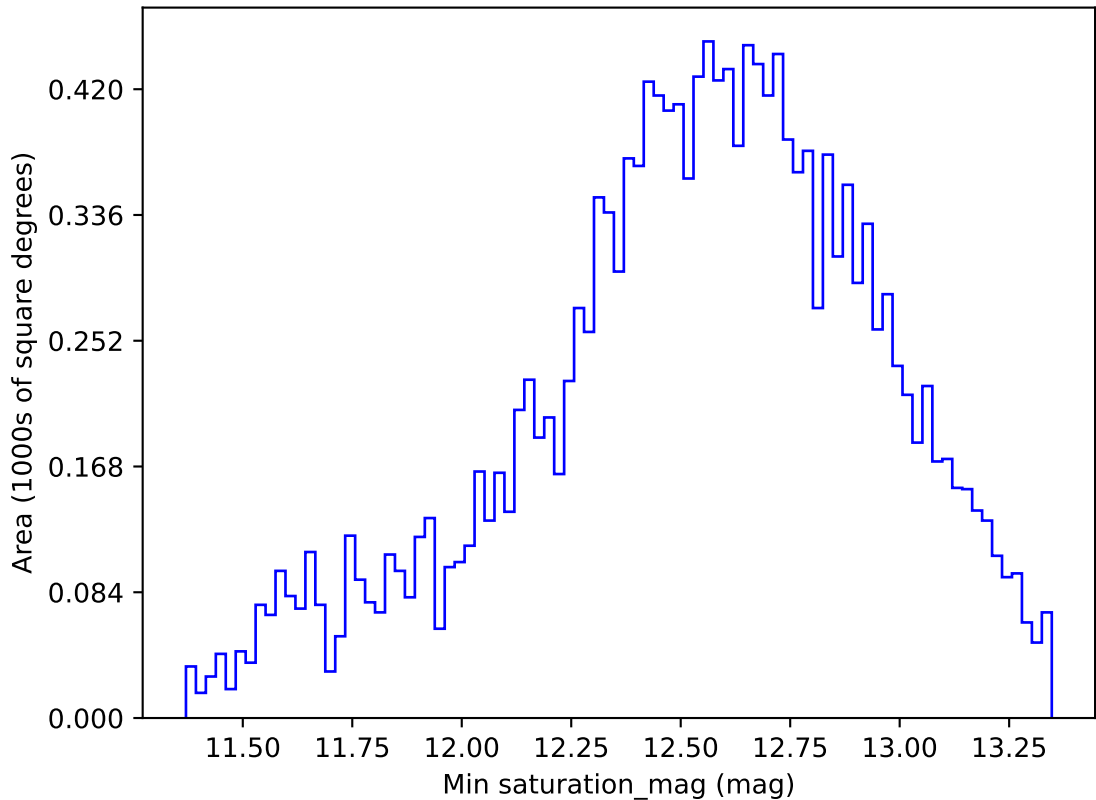
too_combined_s0.5_v3.4_10yrs WFD r band: Min saturation_mag
