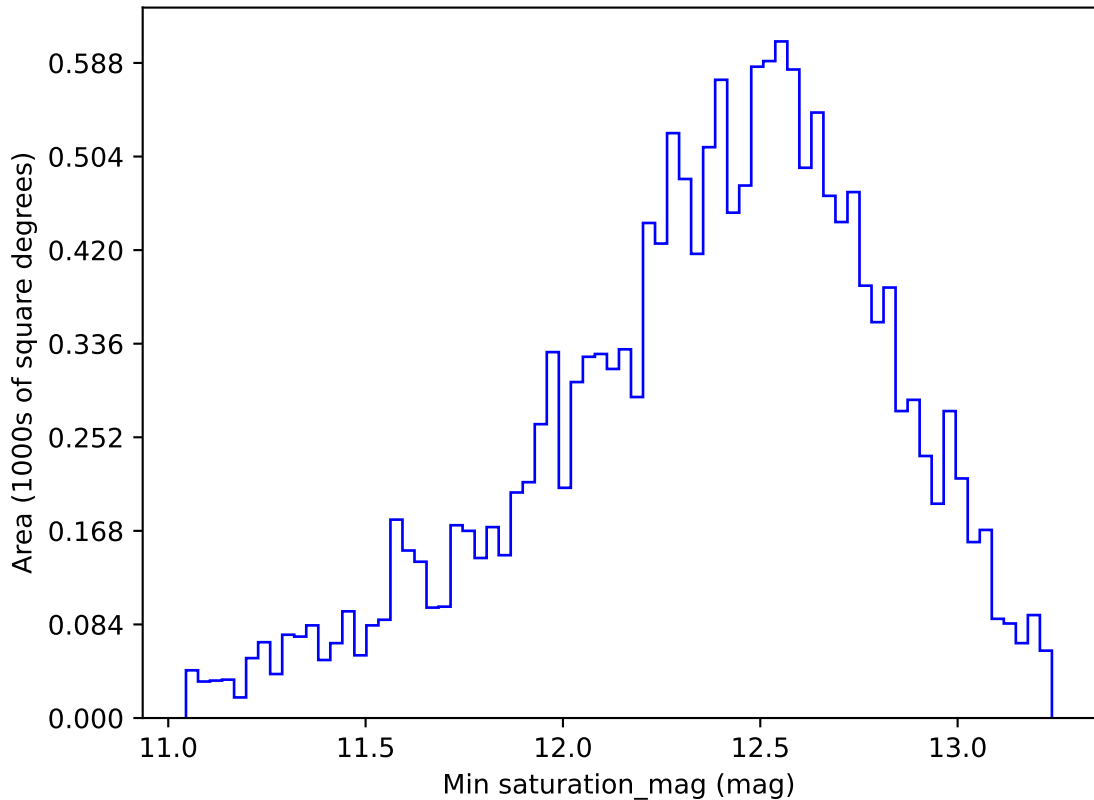
too_combined_s0.5_v3.4_10yrs WFD i band: Min saturation_mag
