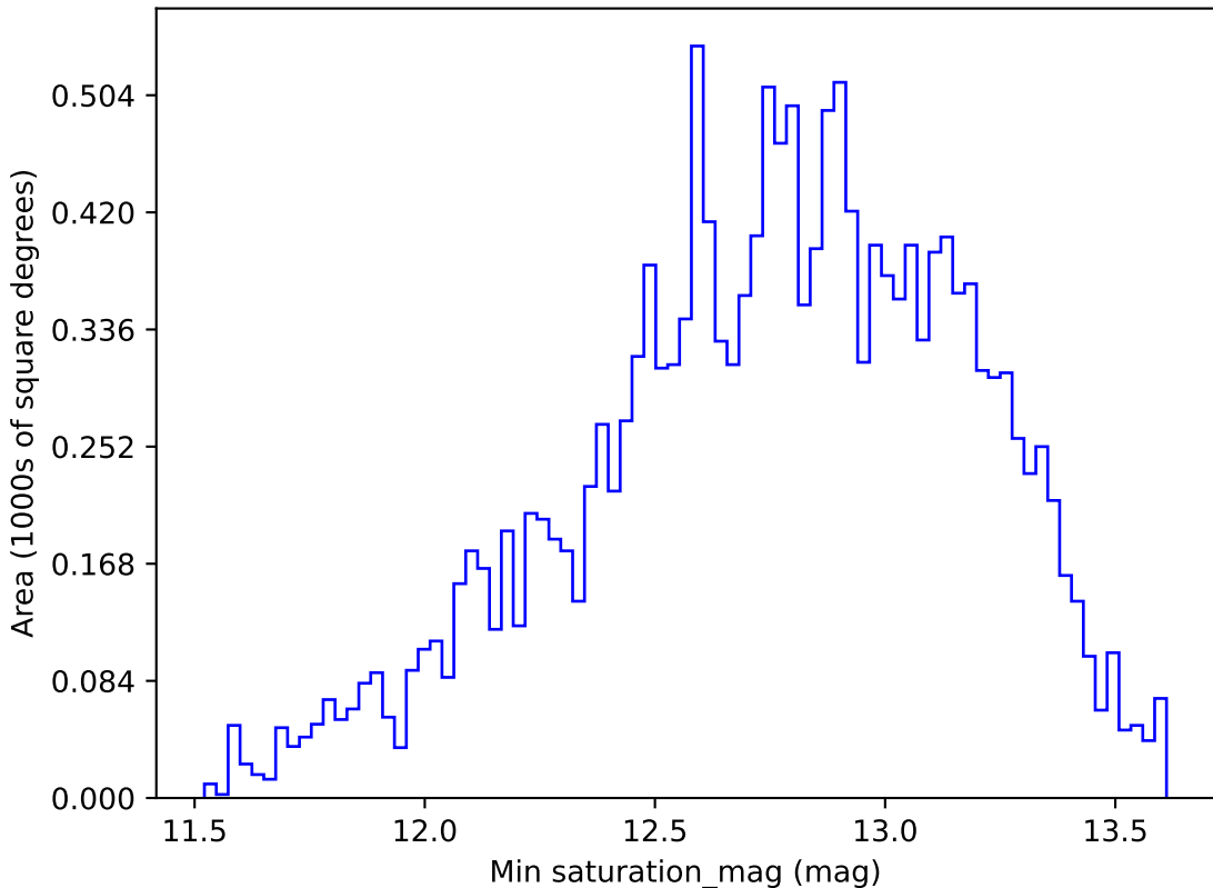
too_combined_s0.5_v3.4_10yrs WFD g band: Min saturation_mag
