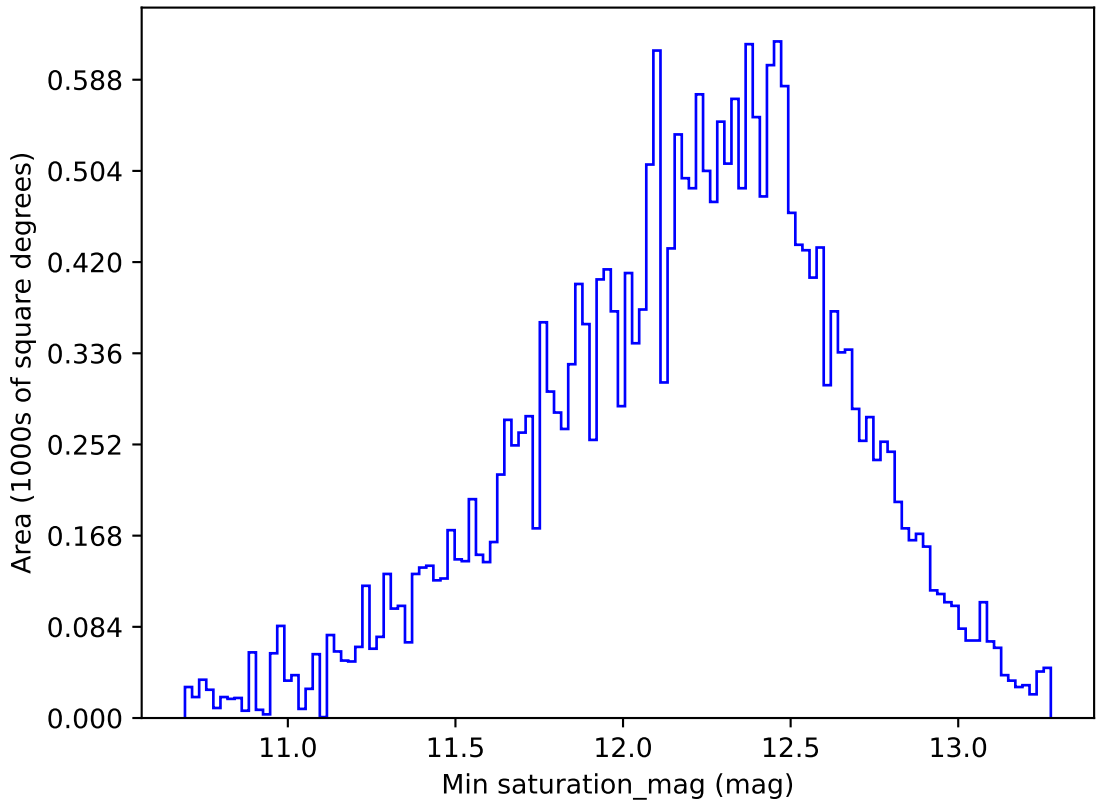
too_combined_s0.5_v3.4_10yrs All sky z band: Min saturation_mag
