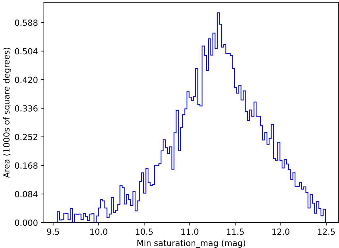
too_combined_s0.5_v3.4_10yrs All sky y band: Min saturation_mag
