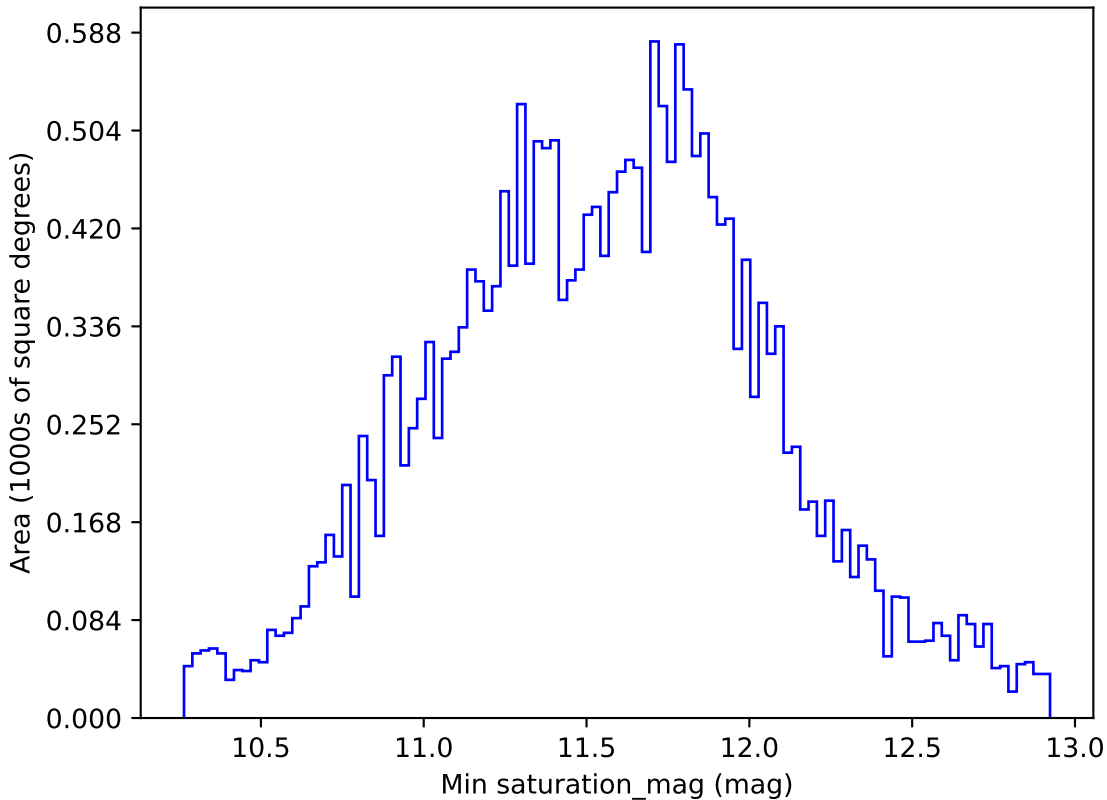
too_combined_s0.5_v3.4_10yrs All sky u band: Min saturation_mag
