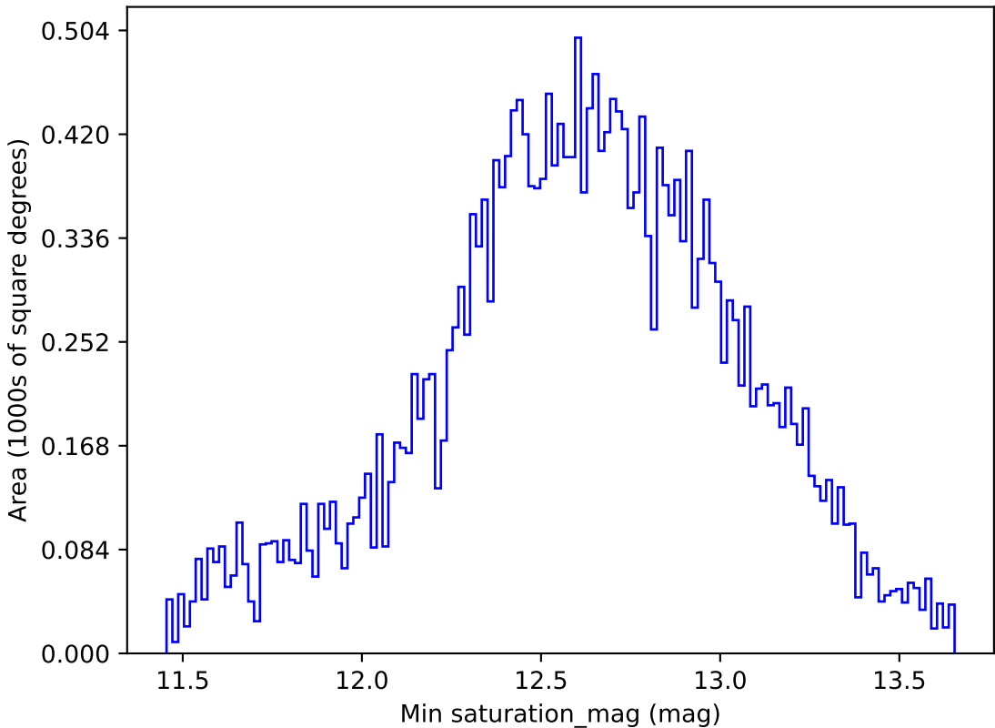
too_combined_s0.5_v3.4_10yrs All sky r band: Min saturation_mag
