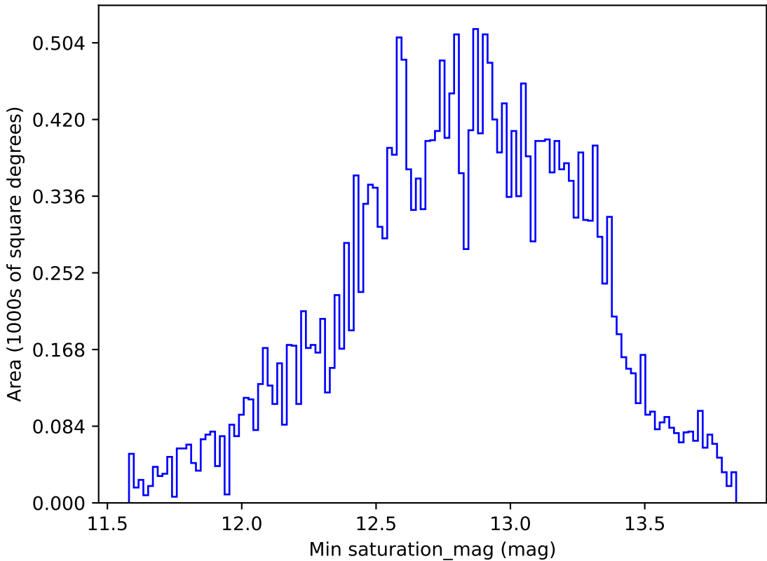
too_combined_s0.5_v3.4_10yrs All sky g band: Min saturation_mag
