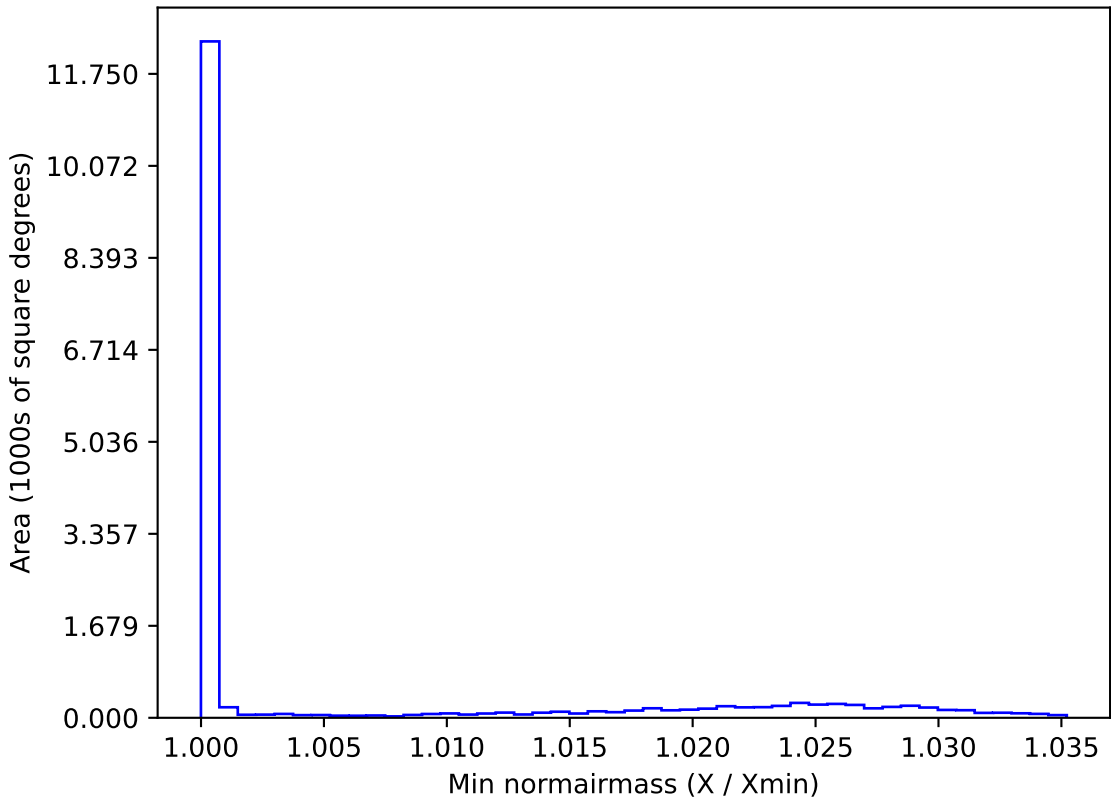
too_combined_s0.5_v3.4_10yrs WFD z band: Min normairmass
