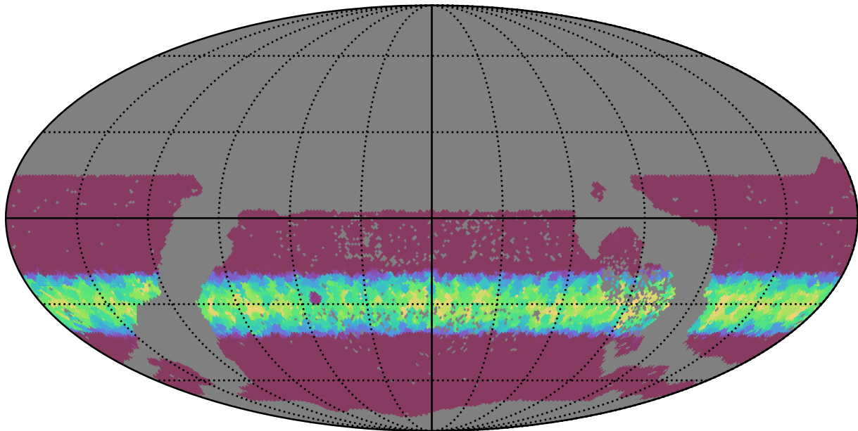
too_combined_s0.5_v3.4_10yrs WFD y band: Min normairmass
