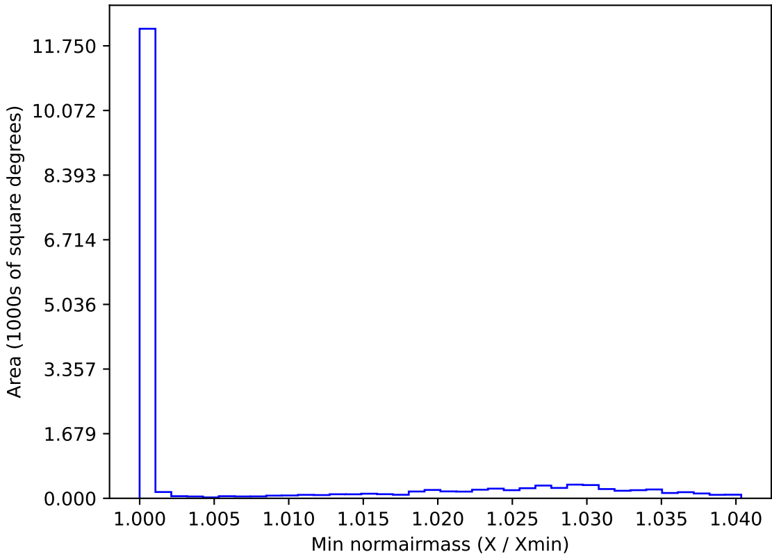
too_combined_s0.5_v3.4_10yrs WFD y band: Min normairmass
