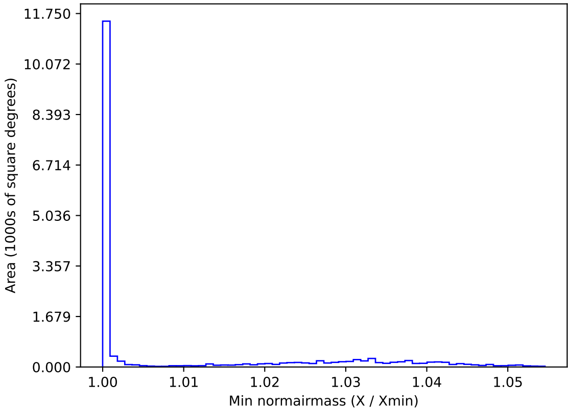
too_combined_s0.5_v3.4_10yrs WFD u band: Min normairmass
