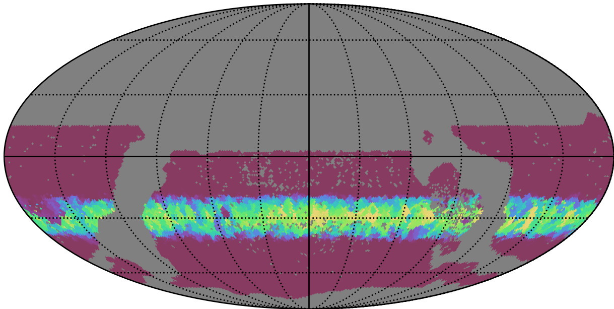
too_combined_s0.5_v3.4_10yrs WFD r band: Min normairmass
