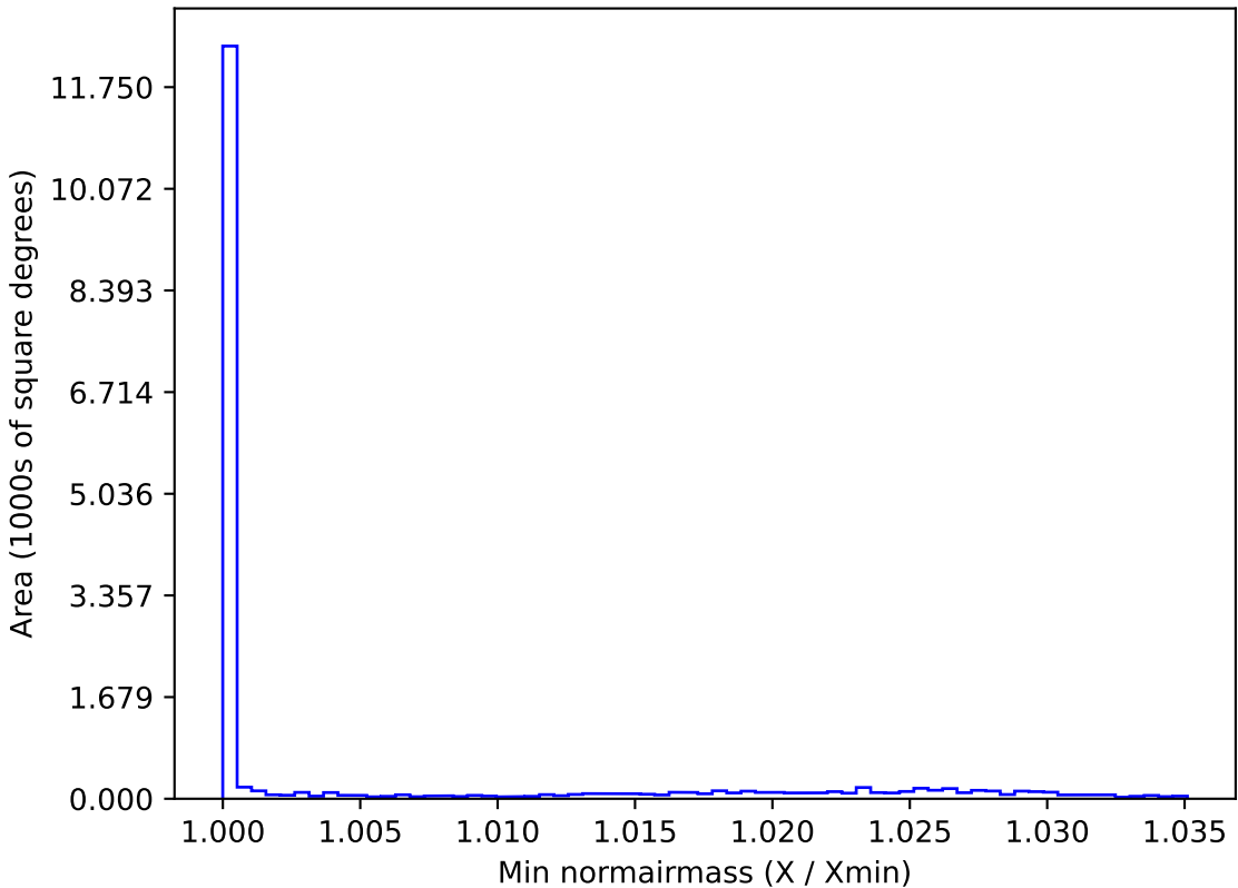
too_combined_s0.5_v3.4_10yrs WFD r band: Min normairmass
