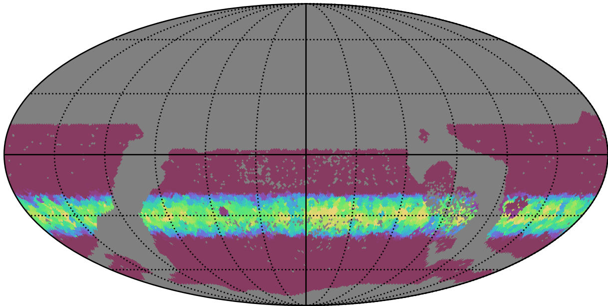
too_combined_s0.5_v3.4_10yrs WFD i band: Min normairmass
