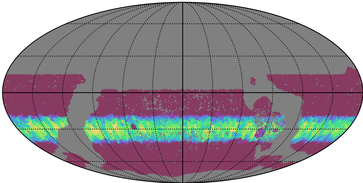
too_combined_s0.5_v3.4_10yrs WFD g band: Min normairmass
