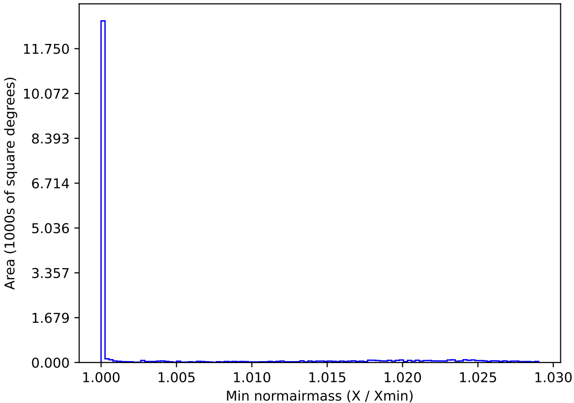
too_combined_s0.5_v3.4_10yrs WFD all bands: Min normairmass
