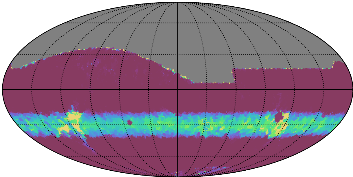
too_combined_s0.5_v3.4_10yrs All sky z band: Min normairmass
