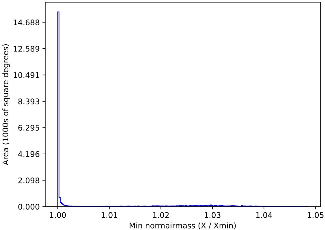
too_combined_s0.5_v3.4_10yrs All sky y band: Min normairmass
