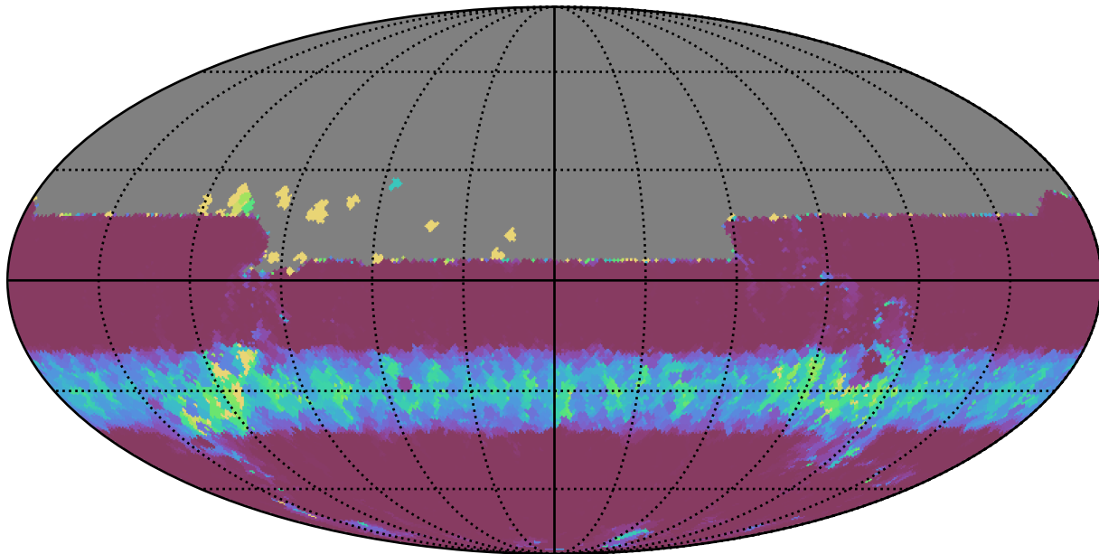
too_combined_s0.5_v3.4_10yrs All sky u band: Min normairmass
