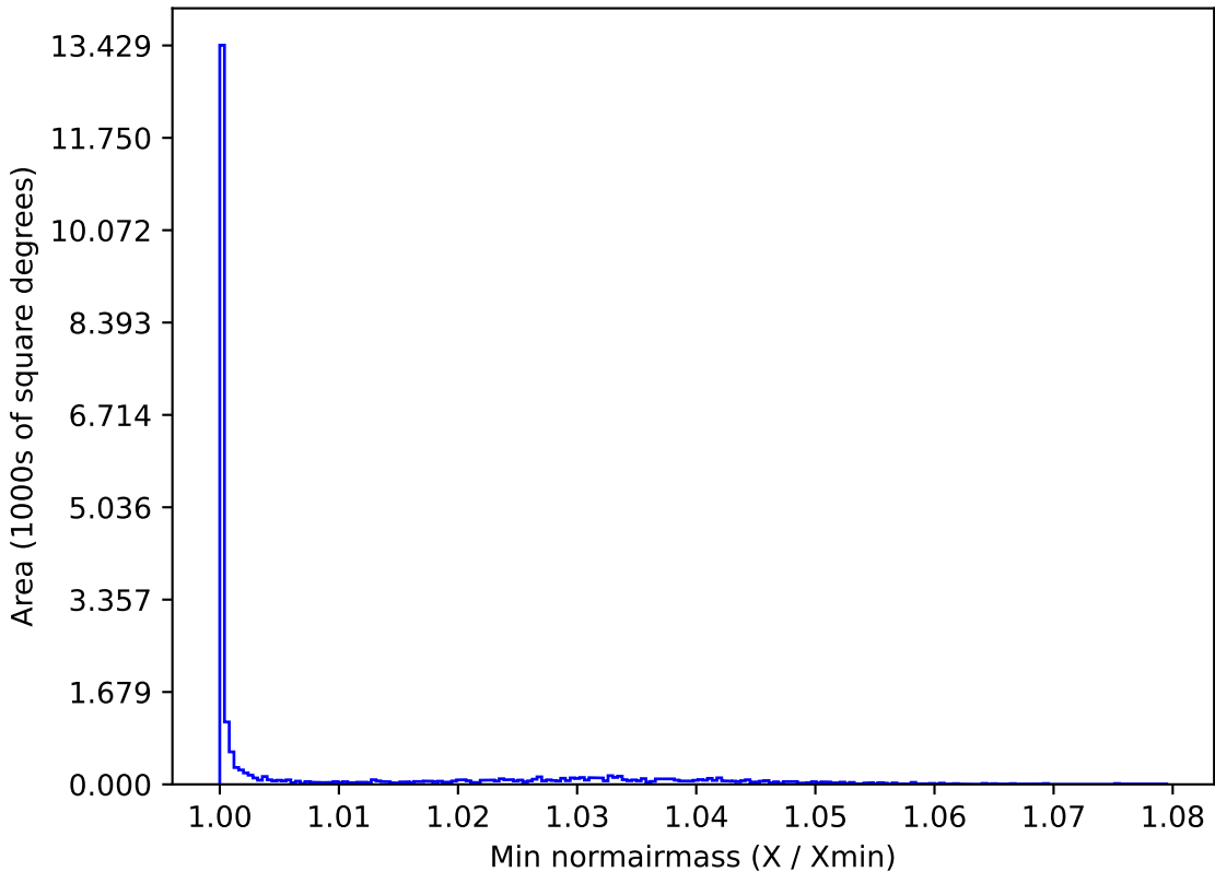
too_combined_s0.5_v3.4_10yrs All sky u band: Min normairmass
