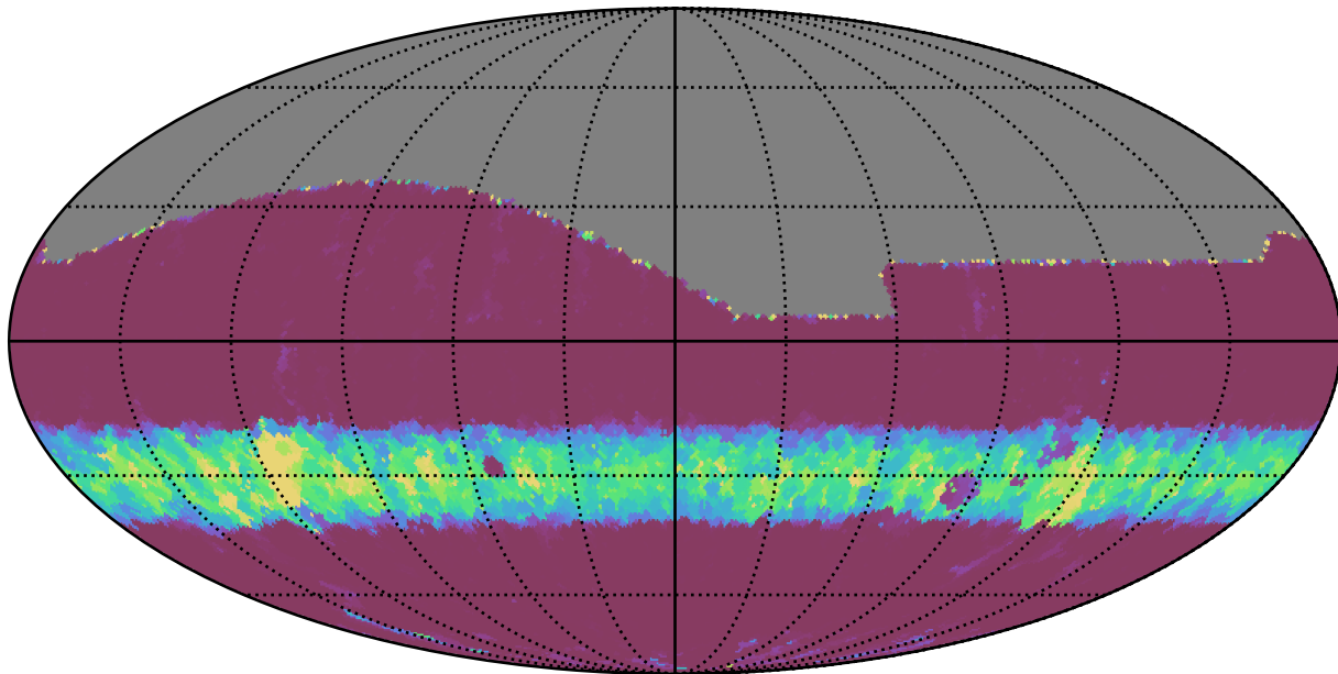
too_combined_s0.5_v3.4_10yrs All sky g band: Min normairmass
