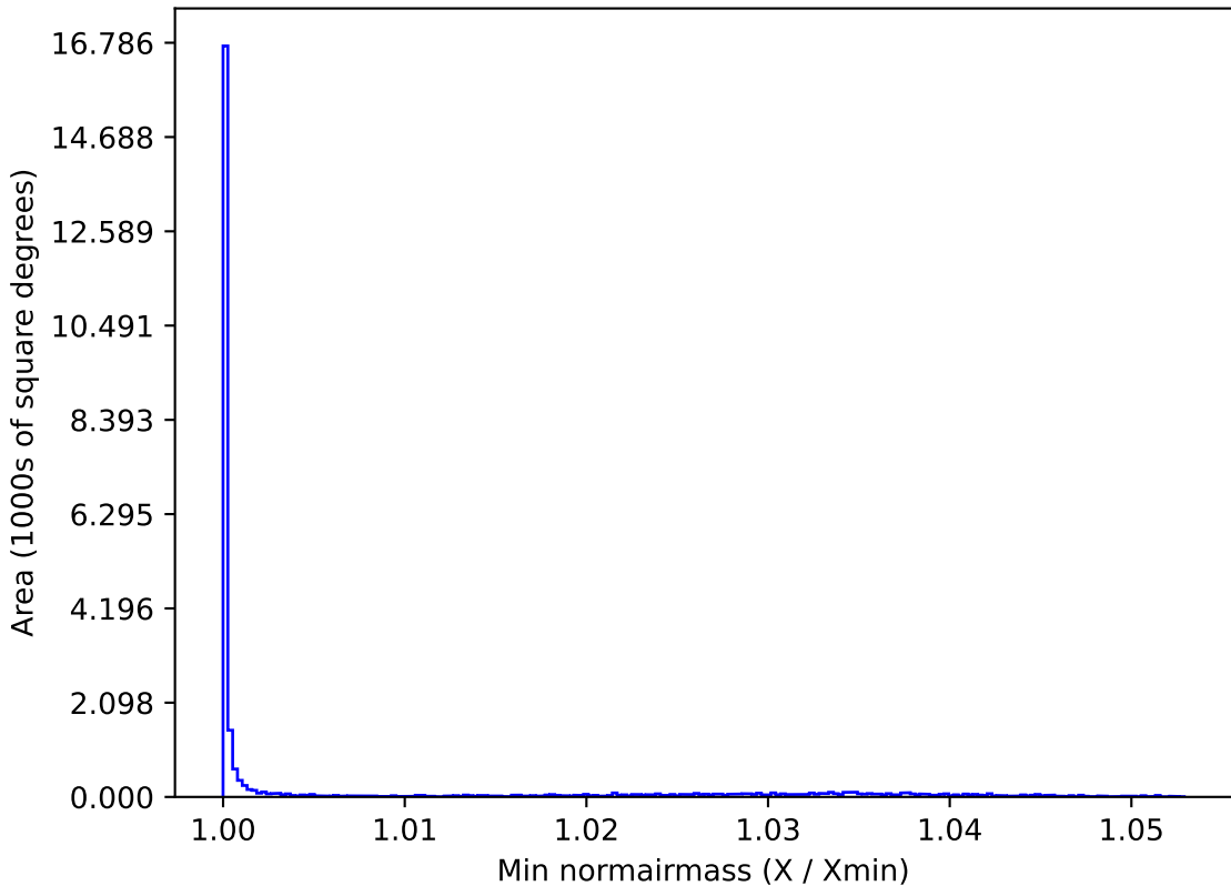
too_combined_s0.5_v3.4_10yrs All sky g band: Min normairmass
