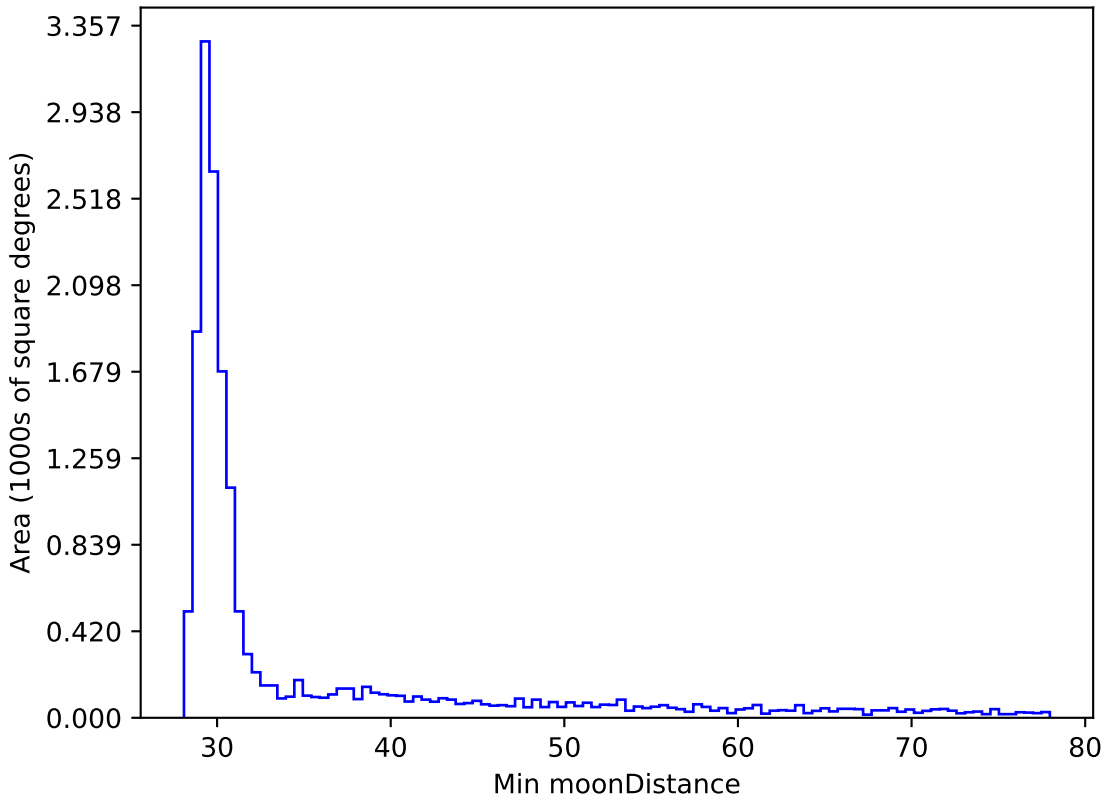
too_combined_s0.5_v3.4_10yrs WFD z band: Min moonDistance
