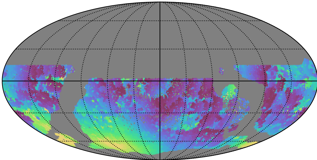
too_combined_s0.5_v3.4_10yrs WFD u band: Min moonDistance
