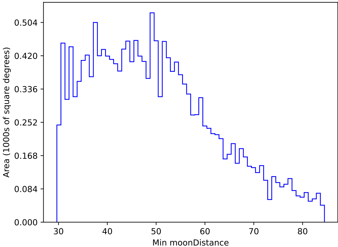
too_combined_s0.5_v3.4_10yrs WFD u band: Min moonDistance
