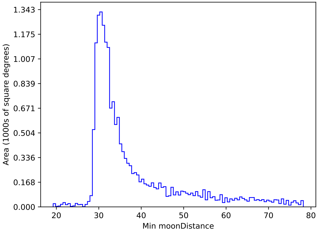
too_combined_s0.5_v3.4_10yrs WFD r band: Min moonDistance
