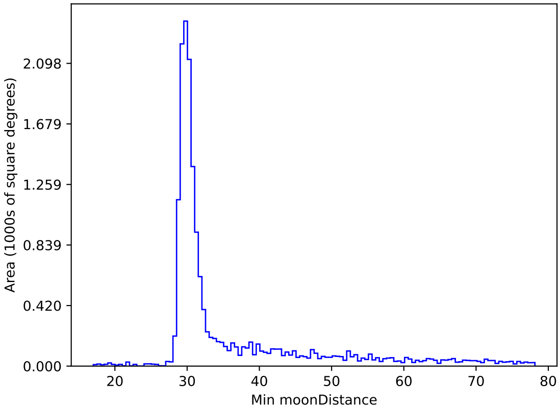
too_combined_s0.5_v3.4_10yrs WFD i band: Min moonDistance
