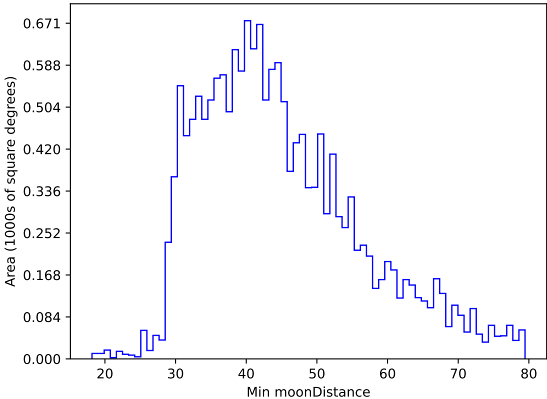
too_combined_s0.5_v3.4_10yrs WFD g band: Min moonDistance
