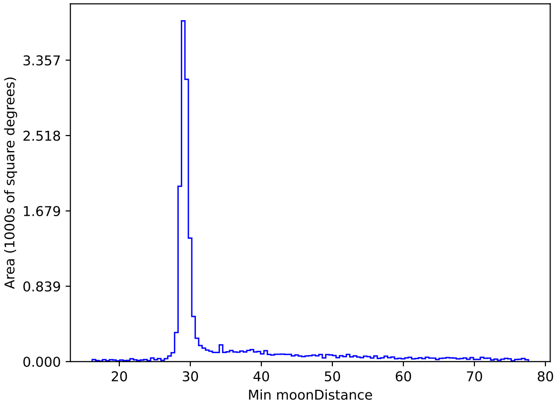
too_combined_s0.5_v3.4_10yrs WFD all bands: Min moonDistance
