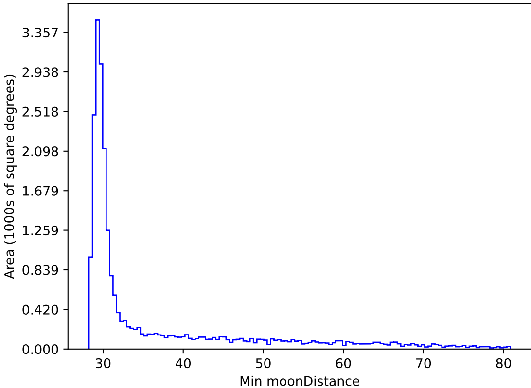
too_combined_s0.5_v3.4_10yrs All sky y band: Min moonDistance
