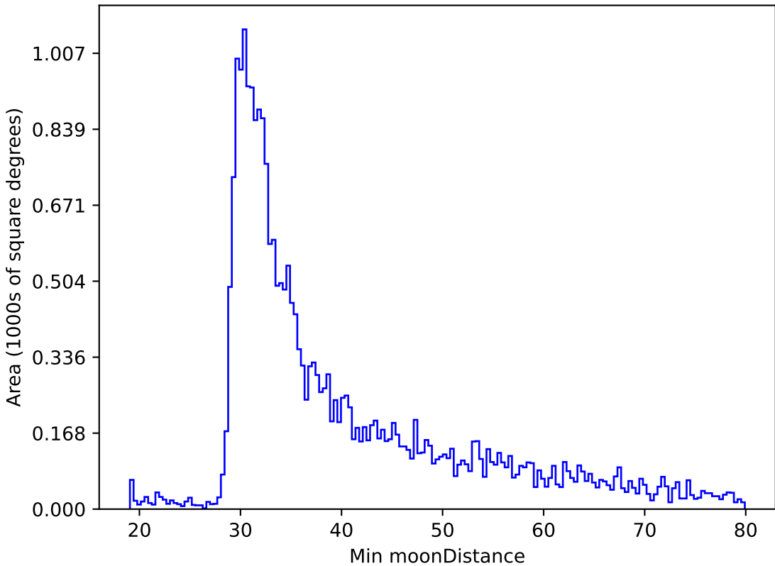
too_combined_s0.5_v3.4_10yrs All sky r band: Min moonDistance
