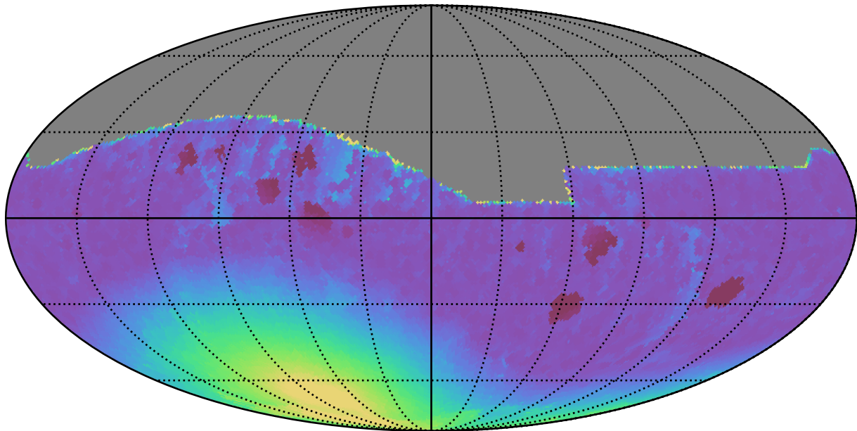
too_combined_s0.5_v3.4_10yrs All sky i band: Min moonDistance
